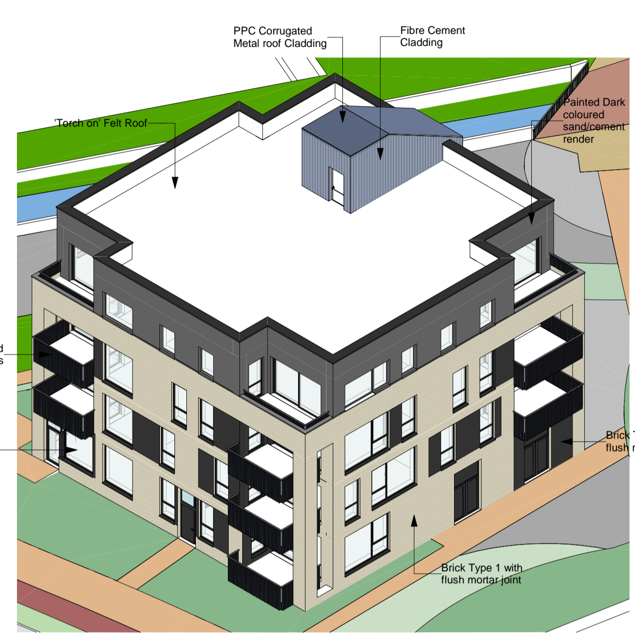
6 3D View 02
