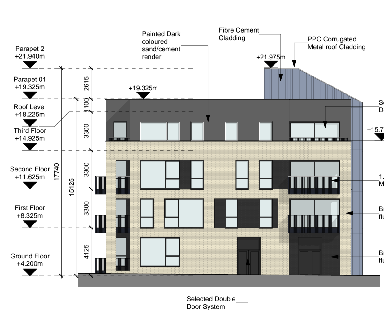
3 East Elevation 1 : 200
