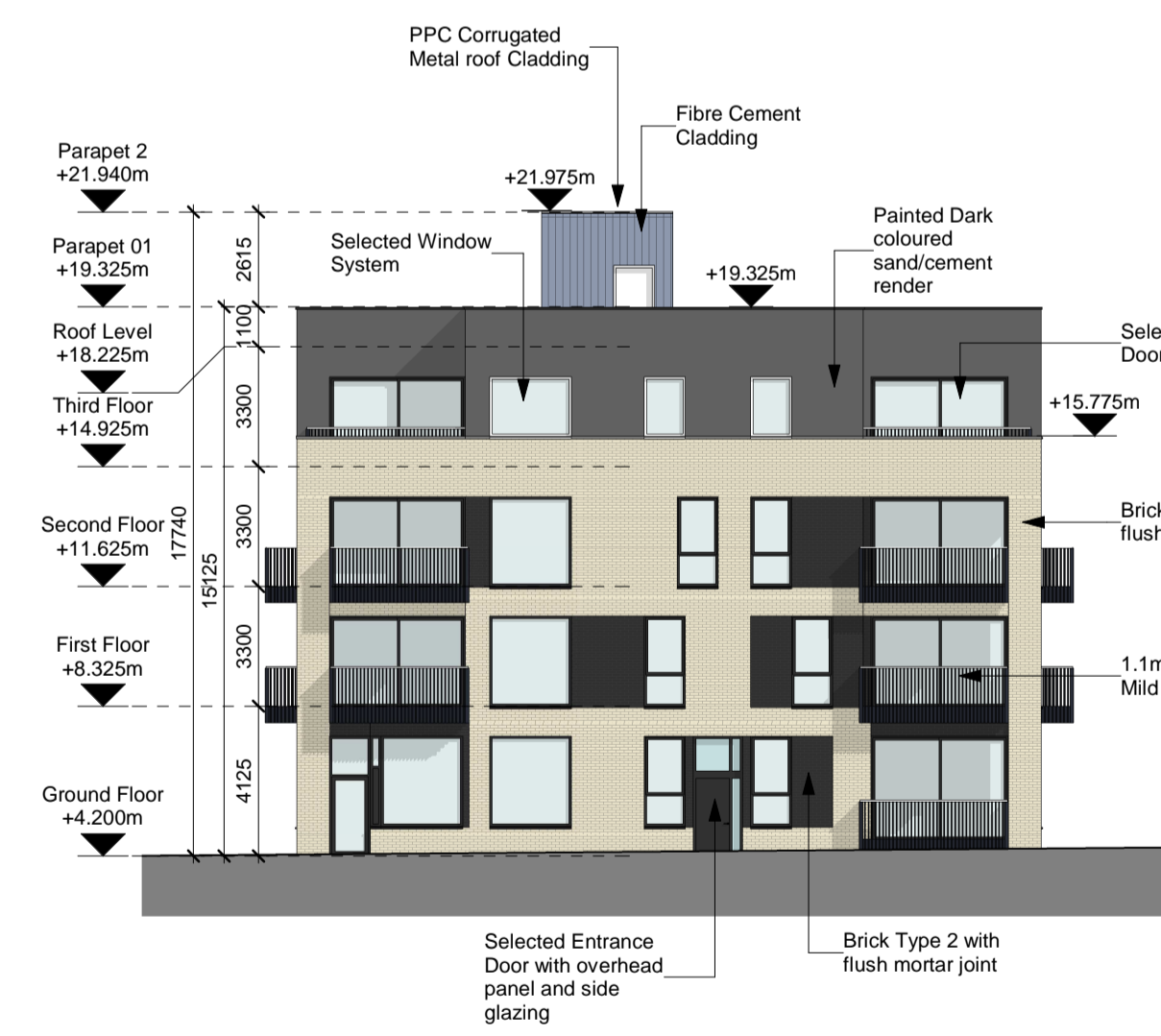
1 South Elevation 1 : 200
