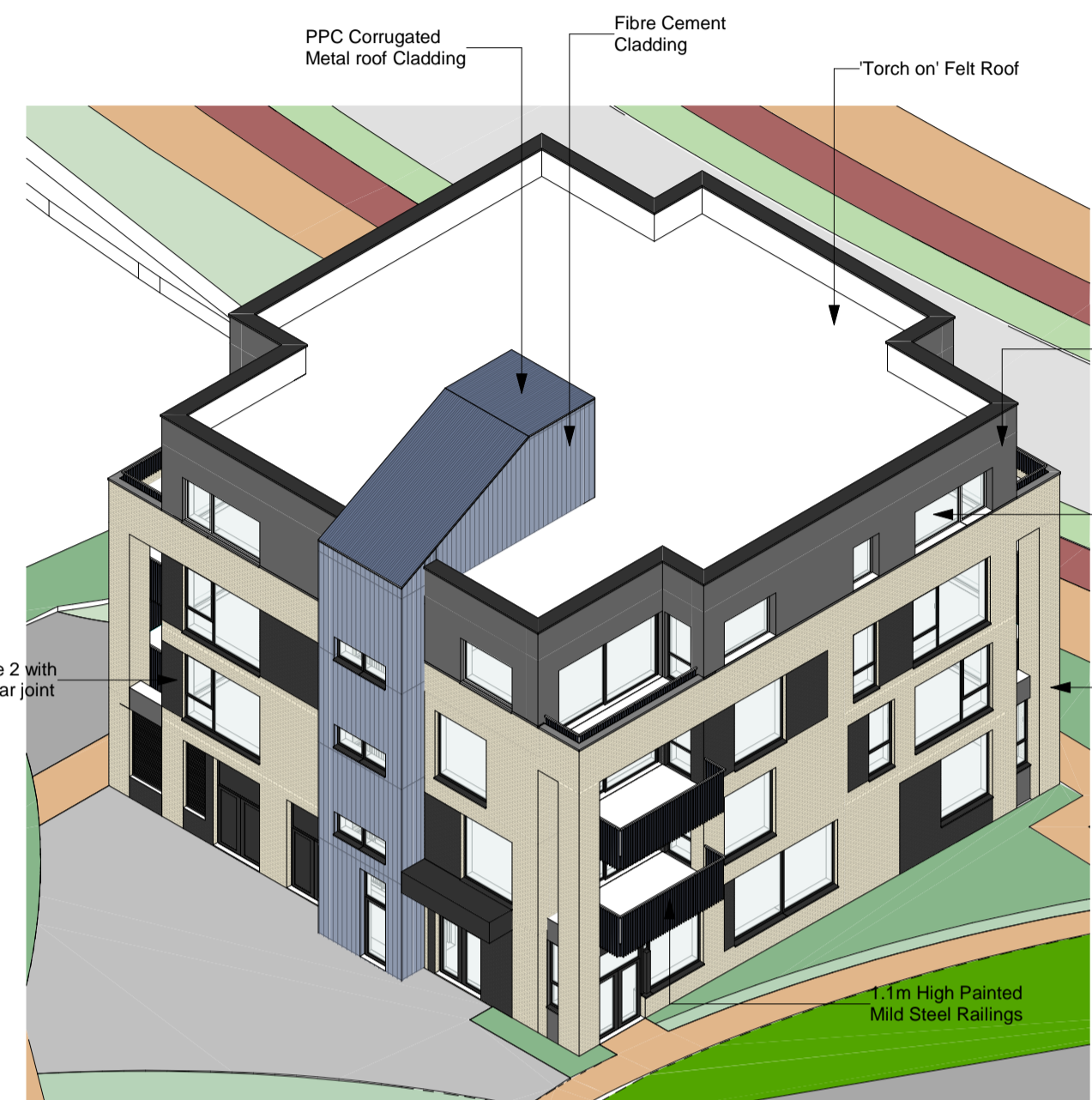
5 3D View 01
